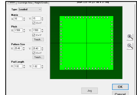
LEADED COMPONENTS
